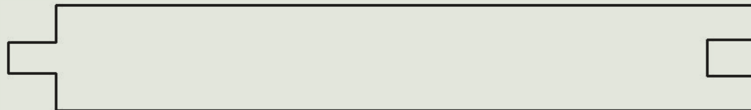
Profile No. 404 144mm x 20.5mm
