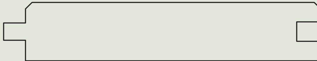
Profile No. 515 145mm x 27mm
