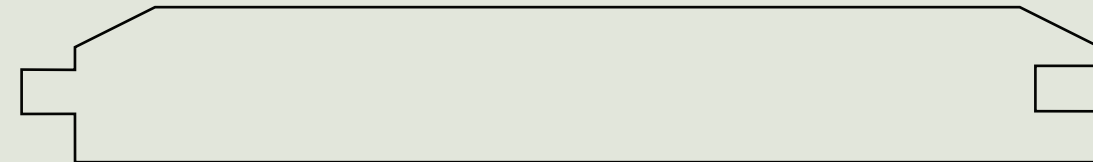
Profile No. 508 142mm x 20.5mm
