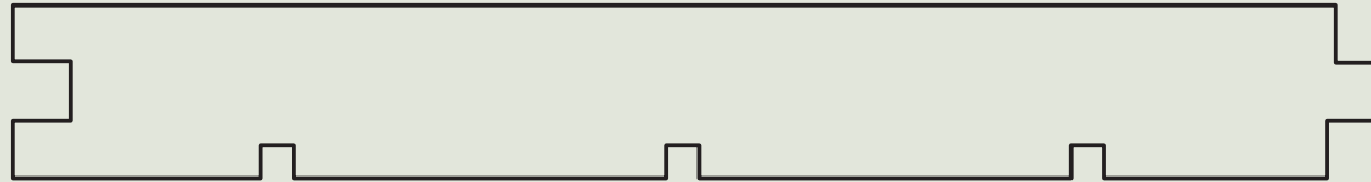
Profile No. 915 160mm x 21mm
