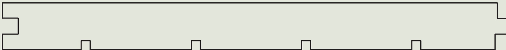
Profile No. 918 220mm x 21mm
