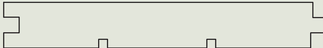
Profile No. 927 140mm x 21mm
